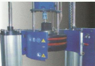
Platen protection system to protect operator from burns and trappings
